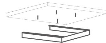
3.Fix semi-finished frame onto ceiling with screw(Concrete ceiling requires plastic anchor)
