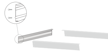
2.Assembling 3 pieces aluminum profile together with screw.
